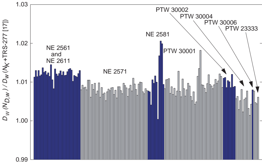
FIG. 19. The ratio of absorbed dose to water in ^{60}\text{Co} determined with calibration factors in terms of absorbed dose to water, N_{D,w} and with calibration factors in terms of air kerma, N_K , using the IAEA TRS-277 [17] Code of Practice for some of the ionization chamber types shown in Fig. 2. Both calibration factors are traceable to the BIPM. The differences are in most cases within the combined standard uncertainty of the two Codes of Practice based on N_{D,w} and N_K .
